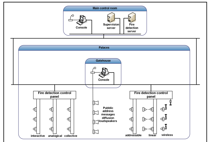
Figure 6. Physical architecture of the fire detection subsystem.
