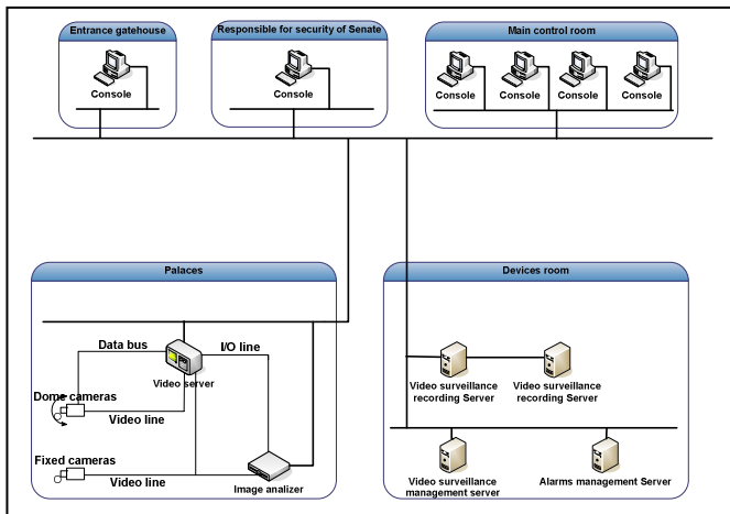
Figure 4. Physical architecture of the video surveillance subsystem.
