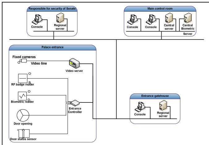
Figure 5. Physical architecture of the access control subsystem.
