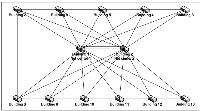
Figure 3. Network architecture schematization.
