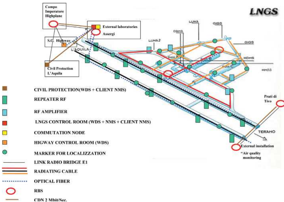
Figure 8: Scheme of the internal radio communication subsystem.
