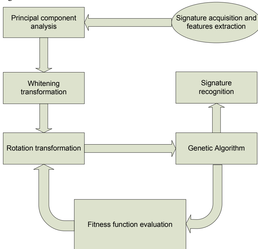
Fig.1 Operative scheme of the system
